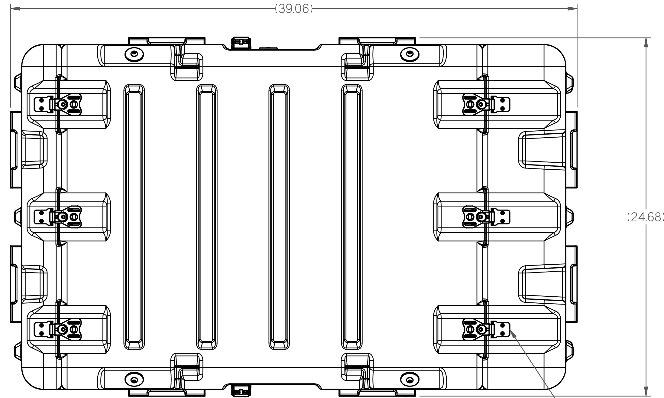
TOP VIEW
