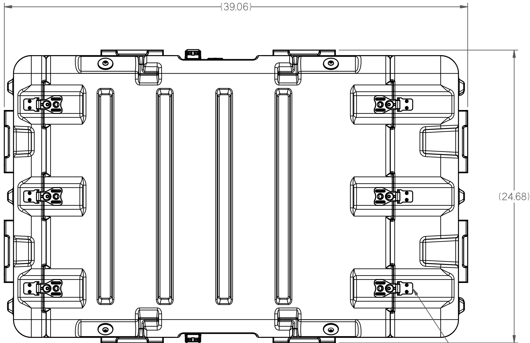
TOP VIEW
