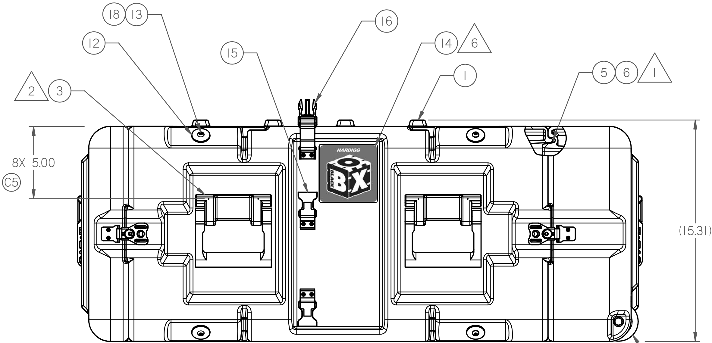
RIGHT SIDE VIEW
